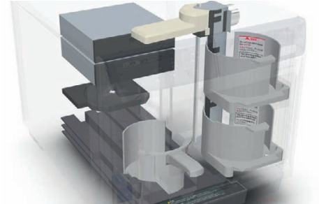
Three trays of 50 discs each allow fully automatic production runs up to 100.
