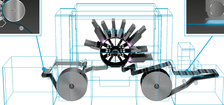
Corona Treater
