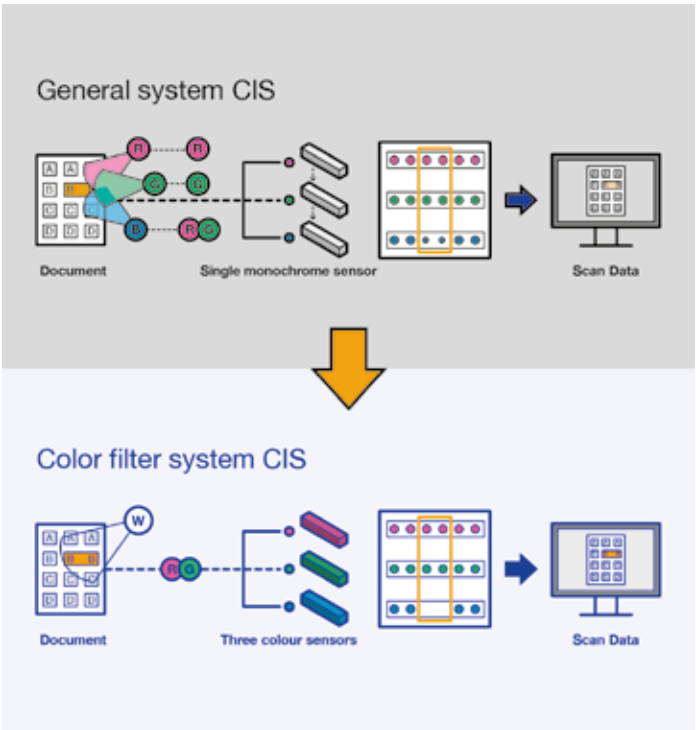
Colour filter system CIS is superior to General system CIS when reading fluorescent colours, especially yellow and orange.
