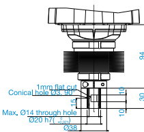
Detail view from "A"
