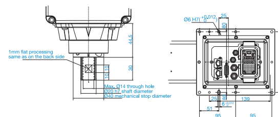
Detail of view "A"
