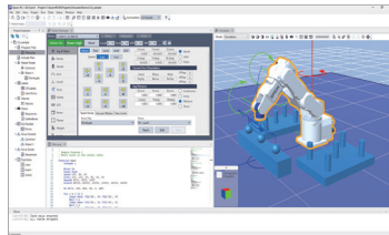
3D simulator for workcell layout and toolpath program testing
