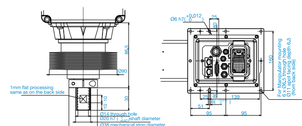
Detail of view "A"
