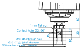
Detail view from "A"
